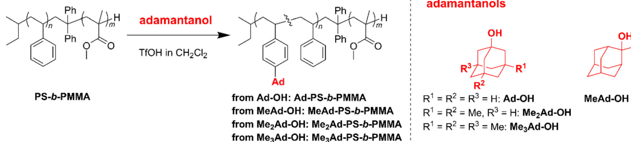
Scheme 1 Metal-free Friedel–Crafts alkylation of PS- b -PMMA using adamantanol.
