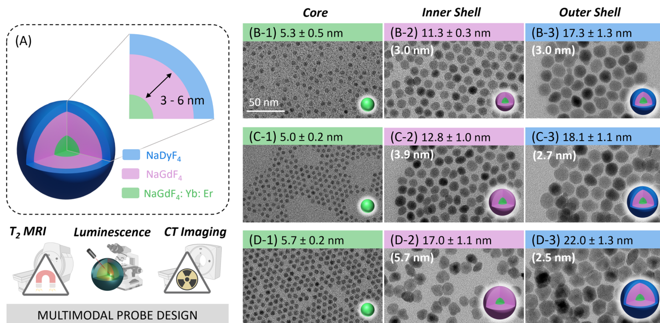
Fig. 1 (A) Schematic illustration of the core/shell/shell Dy-NP architecture proposed as multimodal optical/T 2 /CT probe. (B–D) TEM images and sizes of OA-capped (1) core \beta -NaGdF 4 :Yb,Er, (2) core/shell \beta -NaGdF 4 :Yb,Er/NaGdF 4 , and (3) core/shell/shell \beta -NaGdF 4 :Yb,Er/NaGdF 4 /NaDyF 4 NPs. The NaGdF 4 inner shell thickness and NaDyF 4 outer shell thickness are indicated in brackets. Core sizes and outer shell thicknesses were kept comparable, while the thickness of the inner shell increased from (B) to (D). The 50 nm scale bar applies to all TEM images.
