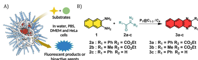
Fig. 3 (A) Representation of reaction involving two substrates using catalytic polymeric nanoparticles; (B) formation of benzoquinoxalines 3a–c initiated by NH insertion followed by intramolecular cyclisation.
