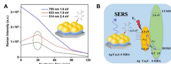
Fig. 10 (A) Intensity of Raman peak at 1586 \text{cm}^{-1} of 4-MBA on Ag/ \text{Cu}_2\text{S} hemispherical dual-shell with various excitation wavelengths and sputtering times and (B) the corresponding coupling scheme in this Ag/ \text{Cu}_2\text{S} /4-MBA system. Reproduced from ref. 195 with permission from American Chemical Society, copyright 2018.
