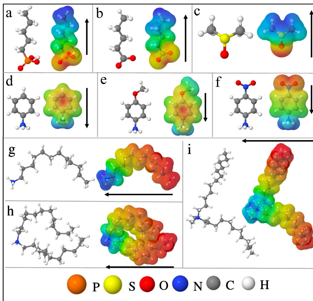
Fig. 1 Molecules and their Hirshfeld charge analysis to show the direction of the dipole moment (a) phosphonate (b) oleate (c) DMSO (d) anilinium (e) anilinium -OCH_3 (f) anilinium -NO_2 . Alkylammonium ligands are taken from classical MD simulation snapshots of ref. 42: (g) primary dodecylammonium (DA) (h) secondary didodecylammonium (DDA), and (i) quaternary dimethyldidodecylammonium (DMDDA). The Red (blue) region corresponds to excess electronic charge (electron deficiency). Black arrows show the direction of the dipole moments (see Fig. S3† for sign convention).
