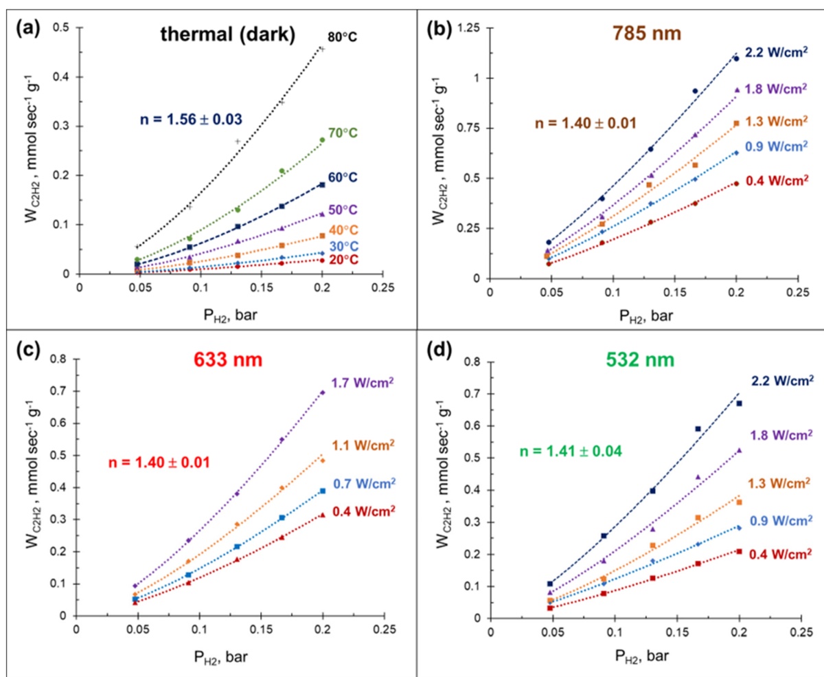
Fig. 4 Acetylene conversion rate over 3%Pd–Mg/GS as a function of hydrogen partial pressure P_{H_2} . (a) Thermal (dark) and photo mediated with laser light illumination wavelengths of (b) 785 nm, (c) 633 nm, and (d) 532 nm. The P_{C_2H_2} was kept constant at 0.05 bar and the reaction order ( n ) reported is with respect to H_2 .
