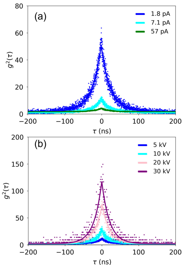
Fig. 4 (a) Current dependence at 5 kV accelerating voltage and (b) accelerating voltage dependence at \sim 10 pA of g^2(\tau) for electron beam parked at 30 nm distance from the nanodiamond on the SiO 2 substrate.
