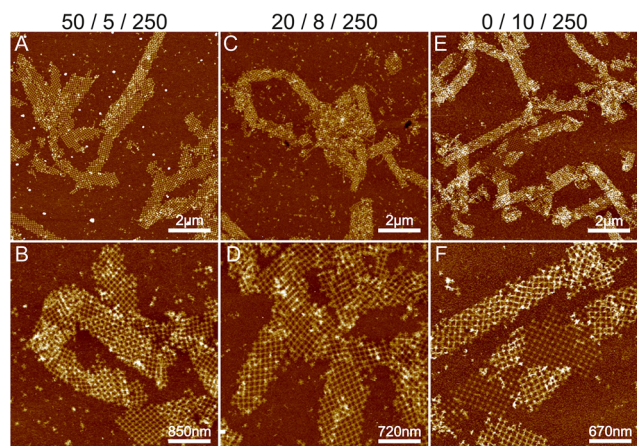
Fig. 2 The effect of nickel on lattice formation. (A and B), (C and D) and (E and F) show AFM images of individual ST depositions when the concentrations C_{Mg^{2+}}/C_{Ni^{2+}}/C_{Na^{+}} are 50/5/250, 20/8/250 and 0/10/250 mM, respectively.
