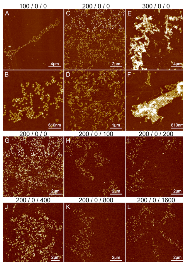
Fig. 1 The effects of \text{Mg}^{2+} and \text{Na}^+ ions on lattice formation. The buffer conditions are listed on top of the images as: C_{\text{Mg}^{2+}}/C_{\text{Na}^{2+}}/C_{\text{Na}^+} . (A and B), (C and D) and (E and F) show the AFM images of STs deposited in 1\times TAE and either 100 mM, 200 mM or 300 mM \text{MgCl}_2 buffer, respectively. (G–L) The effect of \text{Na}^+ ions on lattice formation. The concentration of \text{Mg}^{2+} remains constant at 200 mM while the concentration of \text{Na}^+ is varied between 0 and 1600 mM.
