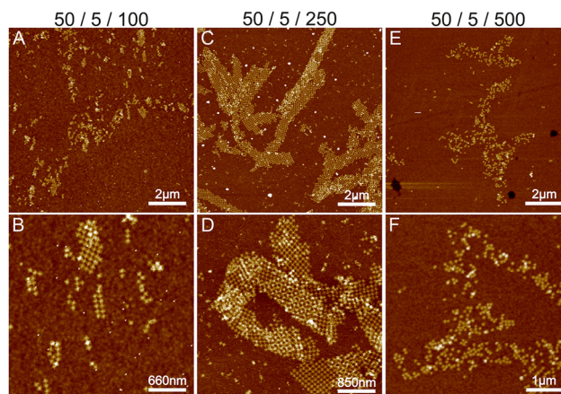
Fig. 3 The combined effect of \text{Mg}^{2+} , \text{Ni}^{2+} and \text{Na}^{+} on lattice formation. (A and B), (C and D) and (E and F) show AFM images of different ST depositions when the concentrations C_{\text{Mg}^{2+}}/C_{\text{Ni}^{2+}}/C_{\text{Na}^{+}} are 50/5/100, 50/5/250 and 50/5/500 mM, respectively.
