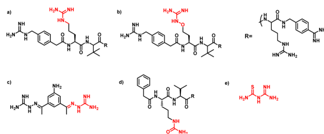
Fig. 1 Chemical structure of furin inhibitors containing (a) guanidine, (b) oxyguanidine, (c) guanyltiourea and (d) urea units. (e) Structure of the guanyltiourea moiety (molecular fragment in the present study).
