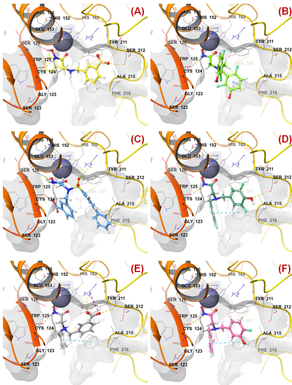
Fig. 9 (A) Binding mode of interaction of compound 47 at the meprin \beta active site (PDB ID: 7AQ1); (B) Binding mode of interaction of compound 55 at the meprin \beta active site (PDB ID: 7AQ1); (C) Binding mode of interaction of compound 38 at the meprin \beta active site (PDB ID: 7AQ1); (D) Binding mode of interaction of compound 13 at the meprin \beta active site (PDB ID: 7AQ1); (E) Binding mode of interaction of compound 7 at the meprin \beta active site (PDB ID: 7AQ1); (F) Binding mode of interaction of compound 37 at the meprin \beta active site (PDB ID: 7AQ1).
