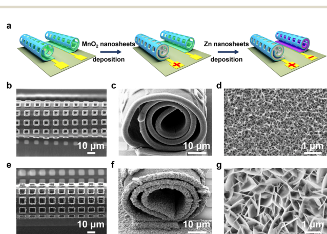
Fig. 2 Manufacture of mesostructured Swiss-roll microelectrodes. (a) Schematic of the Zn– \text{MnO}_2 Swiss-roll microbattery fabrication process. Top (b) and side view (c) SEM images of mesostructured Swiss-roll microcathode. (d) Magnified SEM image of the \text{MnO}_2 morphology. Top (e) and side (f) view of mesostructured Swiss-roll microanode. (g) Magnified SEM image of the Zn nanosheet morphology.
