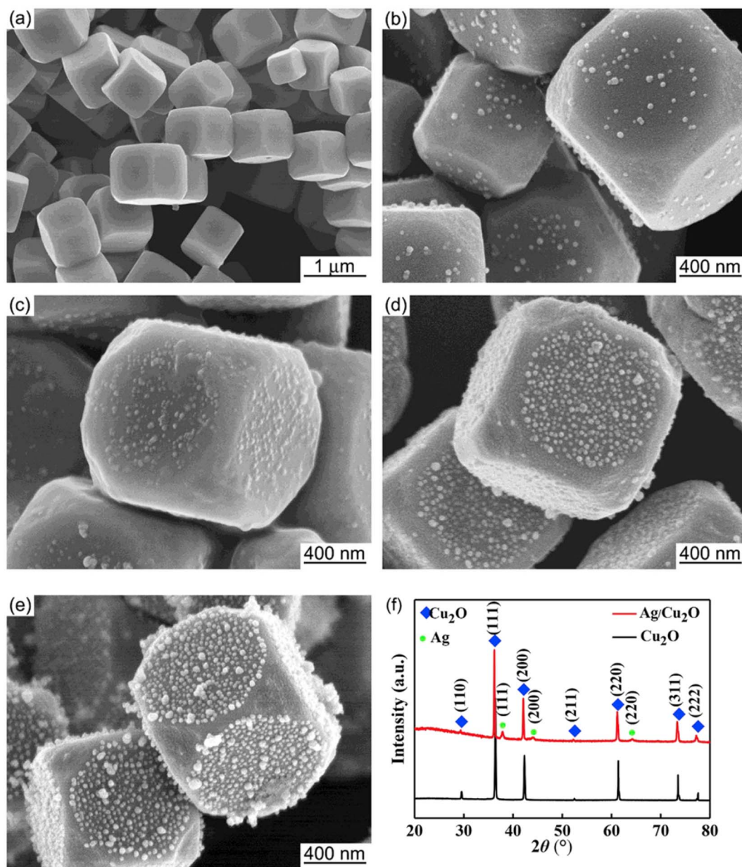
Fig. 2 SEM images of (a) pristine \text{Cu}_2\text{O} and (b–e) \text{Ag} -decorated \text{Cu}_2\text{O} nanostructures, representing a core-satellite structure. The number of \text{Ag} satellites increased with increasing concentration of \text{AgNO}_3 (from (b) to (e)). The XRD patterns for (a) and (e) are shown in (f). Reproduced with permission from ref. 38. Copyright 2019 Elsevier.
