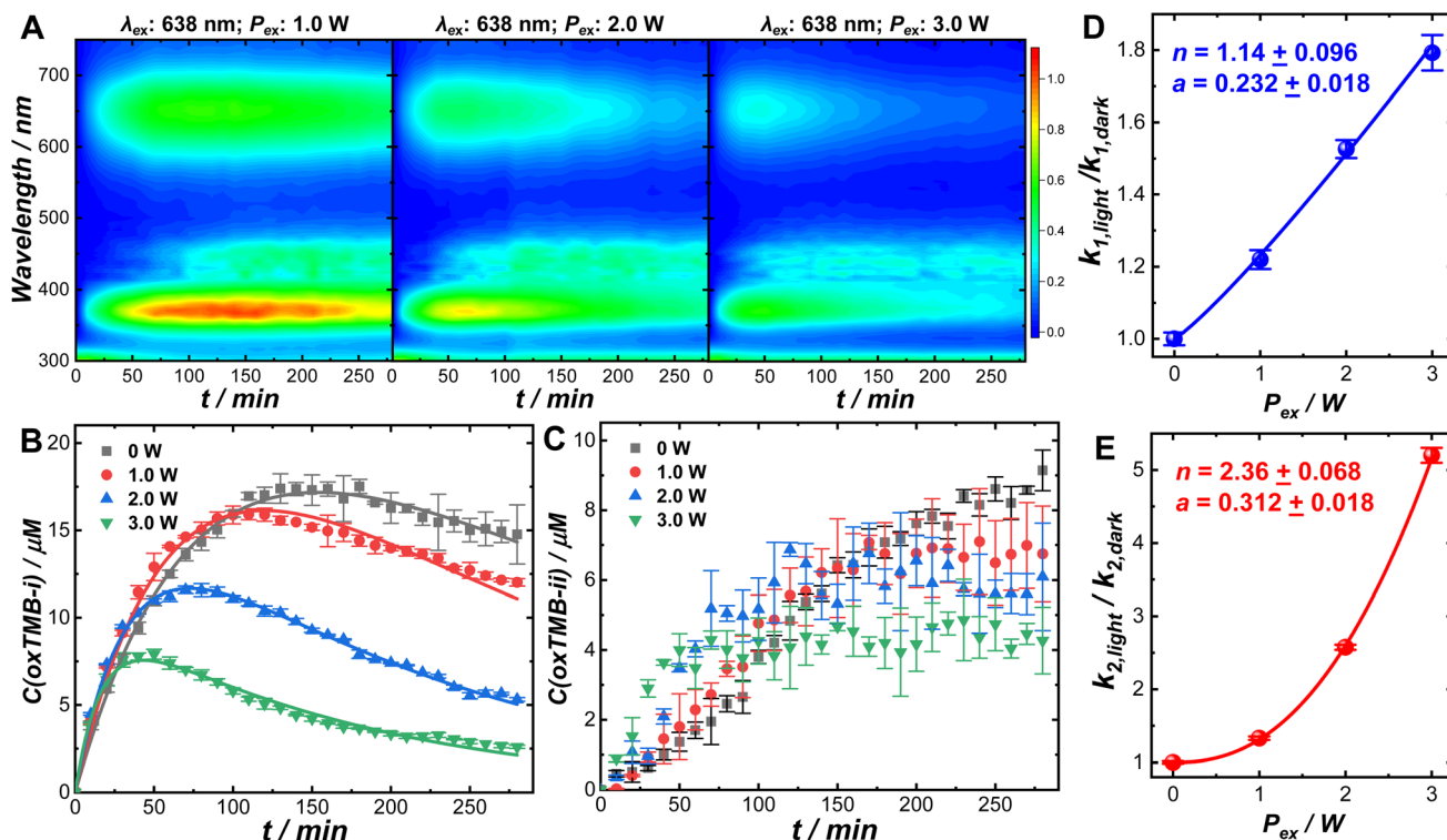
Fig. 3 (A) Time-resolved UV-vis absorption spectra collected during TMB oxidation reactions catalyzed by Au@C/Pt-3 under continuous illumination using a 638 nm laser at P_{ex} s of 1.0, 2.0, and 3.0 W. Temporal evolutions of (B) oxTMB-i and (C) oxTMB-ii concentrations during TMB oxidation catalyzed by Au@C/Pt-3 in the dark and under continuous illumination using a 638 nm laser at P_{ex} s of 1.0, 2.0, and 3.0 W. The initial TMB concentration was 100 \mu\text{M} . The pH of the reaction medium was 8. The total volume of the reactant mixtures was kept at 2.0 mL. The Au@C/Pt-3 nanocatalysts contained 2.33 \mu\text{g} Au in all cases. The reaction temperatures under laser illumination were controlled at 25 \pm 1 ^{\circ}\text{C} using a circulating water bath. The error bars in panels (B) and (C) represent the standard deviations of triplicate kinetic measurements under each reaction condition. The curve fitting results are shown as solid curves in panel (B). P_{ex} -dependence of photo-induced kinetic enhancements (defined as the ratios between the rate constants under light illumination and in the dark) for (D) k_1 and (E) k_2 . The error bars in panels (D) and (E) represent the standard deviations associated with the least squares curve fitting of the kinetic results shown in panel (B). The relationships between rate constants and P_{ex} were fitted with a power function and the fitting results are shown as solid curves in panels (D) and (E).
