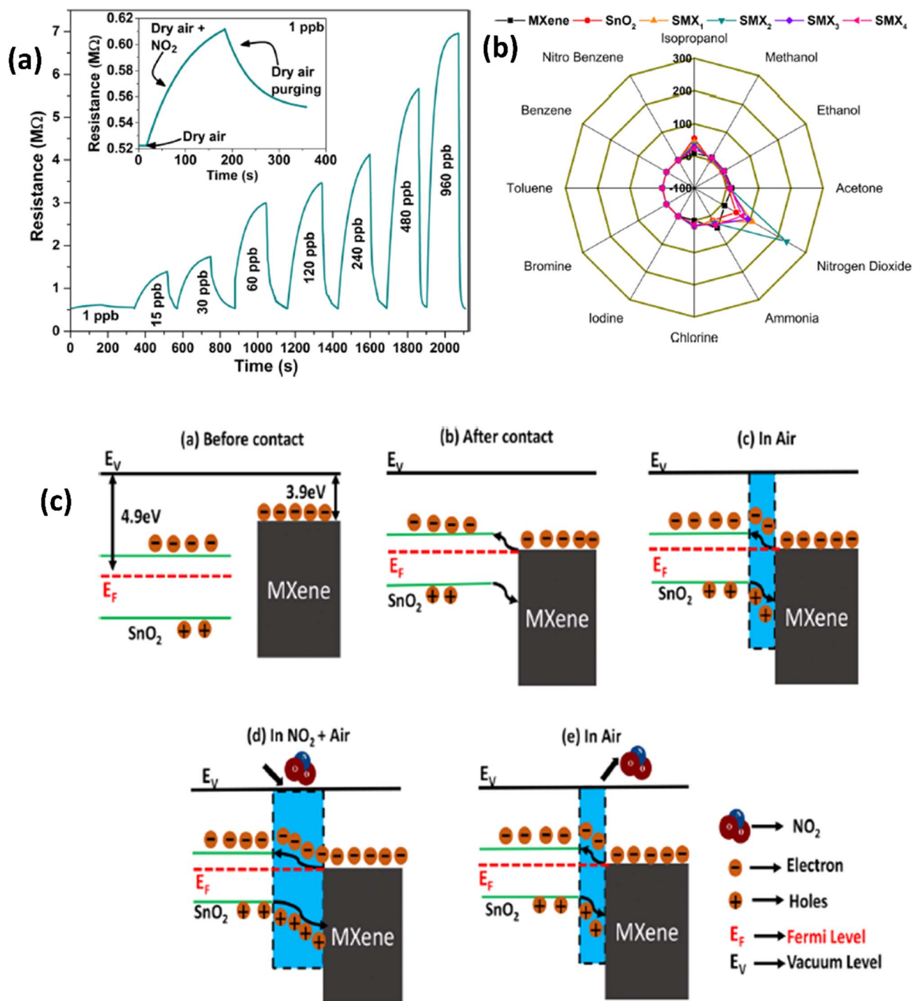
Fig. 4 (a) Resistance–time curves for the SnO 2 /MXene sensor with exposure to different concentrations of NO 2 . (b) Polar plots for various gases at 30 ppb concentrations for pristine SnO 2 , MXenes and their heterostructures at room temperature. (c) Schematic representation of the NO 2 sensing mechanism of the SnO 2 /MXene heterostructure, reprinted in part permission from ref. 60 Copyright (2023) Elsevier.
