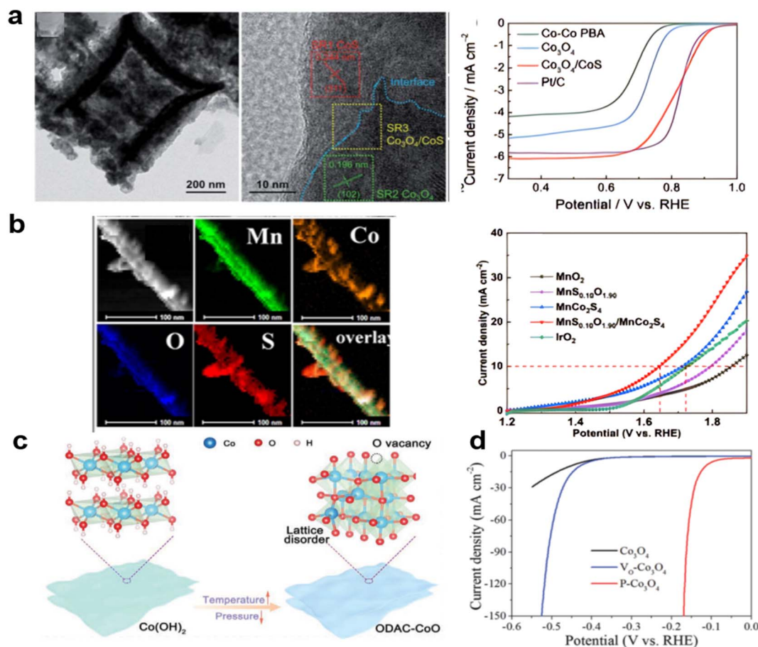
Fig. 9 Heterodoped spinels for high performance: (a) S on Co 3 O 4 derived from PBA, (reproduced from ref. 192 with permission from the Royal Society of Chemistry) (b) S on MnCo 2 O 4 needles, (reproduced from ref. 194 with permission. Copyright © 2021 Elsevier) (c) O vacancies introduced by vacuum heating, (reproduced from ref. 198 with permission. Copyright ©2021 Wiley-VCH) (d) P by plasma treatment (reproduced from ref. 200 with permission from the Royal Society of Chemistry).
