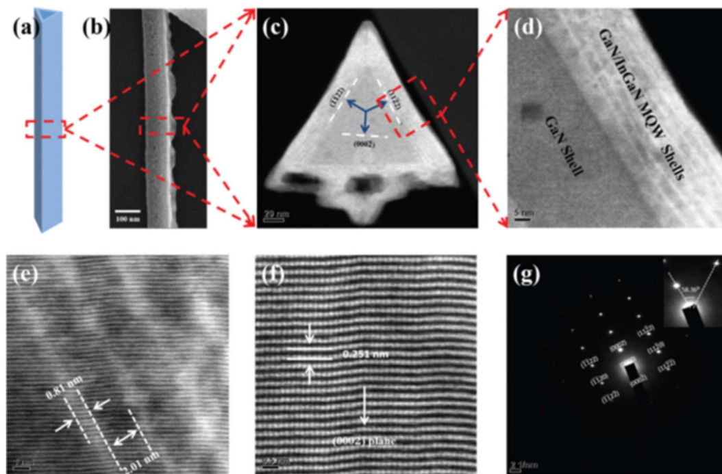
Fig. 3 (a) Schematic illustration of a GaN/InGaM MQW co-axial single NW, (b) low-magnification STEM micrograph, in which the growth direction of GaN core NWs is also shown along the m -axis, (c) cross-sectional HAADF-STEM micrograph of a single NW prepared by FIB, (d) layer-by-layer structure of the GaN/InGaM pairs from one side of an isosceles NW, (e) high-magnification micrograph depicting the InGaM QWs, (f) inter-planar measurement of the structure with QWs, and (g) SAED patterns of the GaN/InGaM disk. Reproduced with permission from ref. 79. Copyright 2019 RSC publisher.
