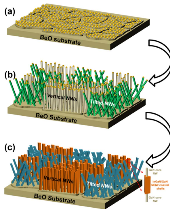
Fig. 4 Depicts a schematic representation of the GaN-based NW fabrication flow: (a) aggregation of the Au/Ga/In metal alloy catalyst, (b) formation of the GaN core NWs, and (c) InGaM/GaN MQW coaxial shells on the BeO substrate; the inset indicates the geometry of the core/shell structure. Reproduced with permission from ref. 81. Copyright 2020 ACS publisher.
