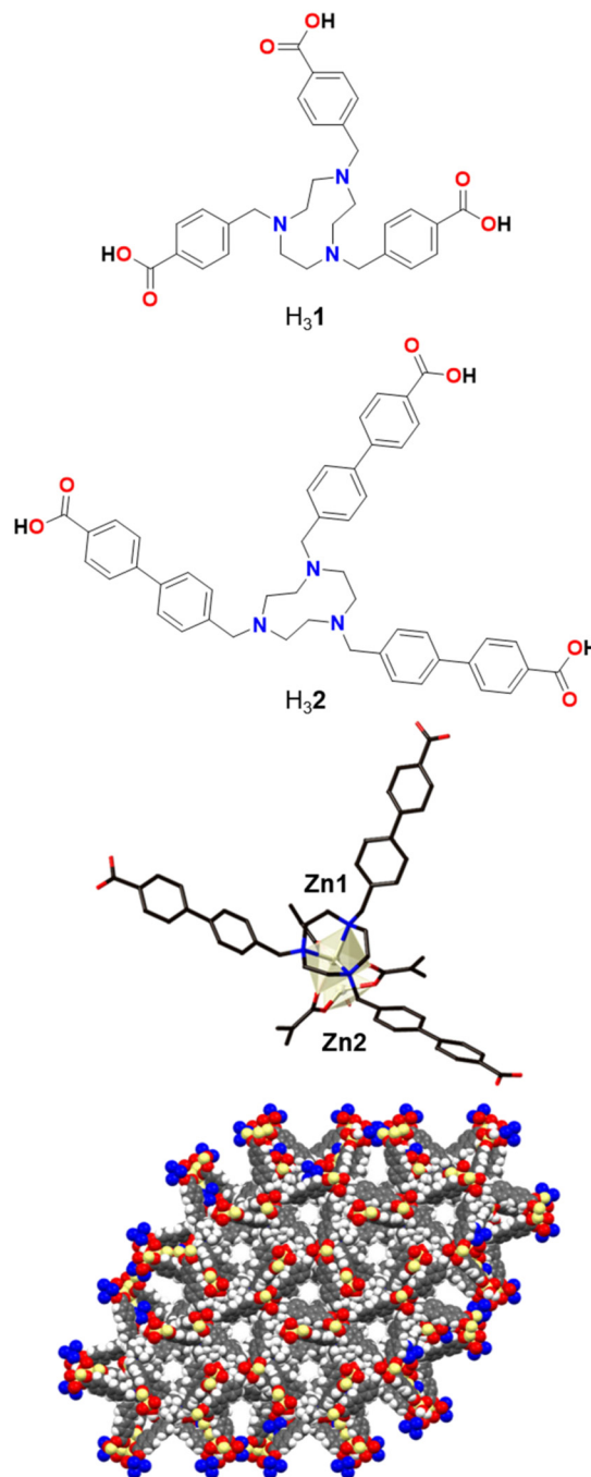
Fig. 1 Designed TACN-based tricarboxylic acid H_32 with extended, rigid arms compared to the previously reported H_31 (top), magnified view of the dinuclear Zn cluster in poly- [\text{Zn}_2(2)(\text{OH}_2)]\text{Cl} (middle), and view of the pore channels along the crystallographic c -axis (bottom).
