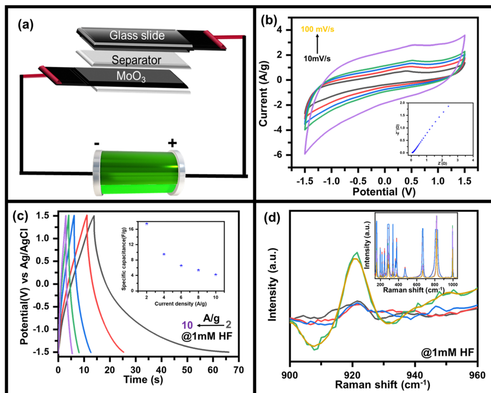
Fig. 4 (a) Schematic diagram of as-fabricated \text{MoO}_3/\text{AC} supercapacitor device, (b) CV curves measured at scan rates of 10 to 100 \text{ mV s}^{-1} along with the corresponding EIS plot (ESI † ), (c) GCD plots at 2 \text{ A g}^{-1} to 10 \text{ A g}^{-1} along with variation of specific capacitance as a function of current density (inset) and (d) in situ Raman spectra of asymmetric supercapacitor device during the charging and discharging process.
