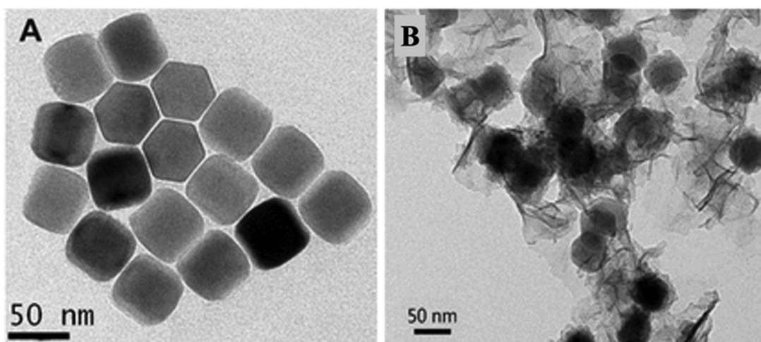
Fig. 13 TEM images (A) of OA-capped \text{NaYF}_4:\text{Yb},\text{Tm}@\text{NaYF}_4 core shell UCNPs, and (B) of \text{MnO}_2 NS-modified \text{NaYF}_4:\text{Yb},\text{Tm}@\text{NaYF}_4 UCNPs assemblies. 67 Copyright©2015, American Chemical Society.
