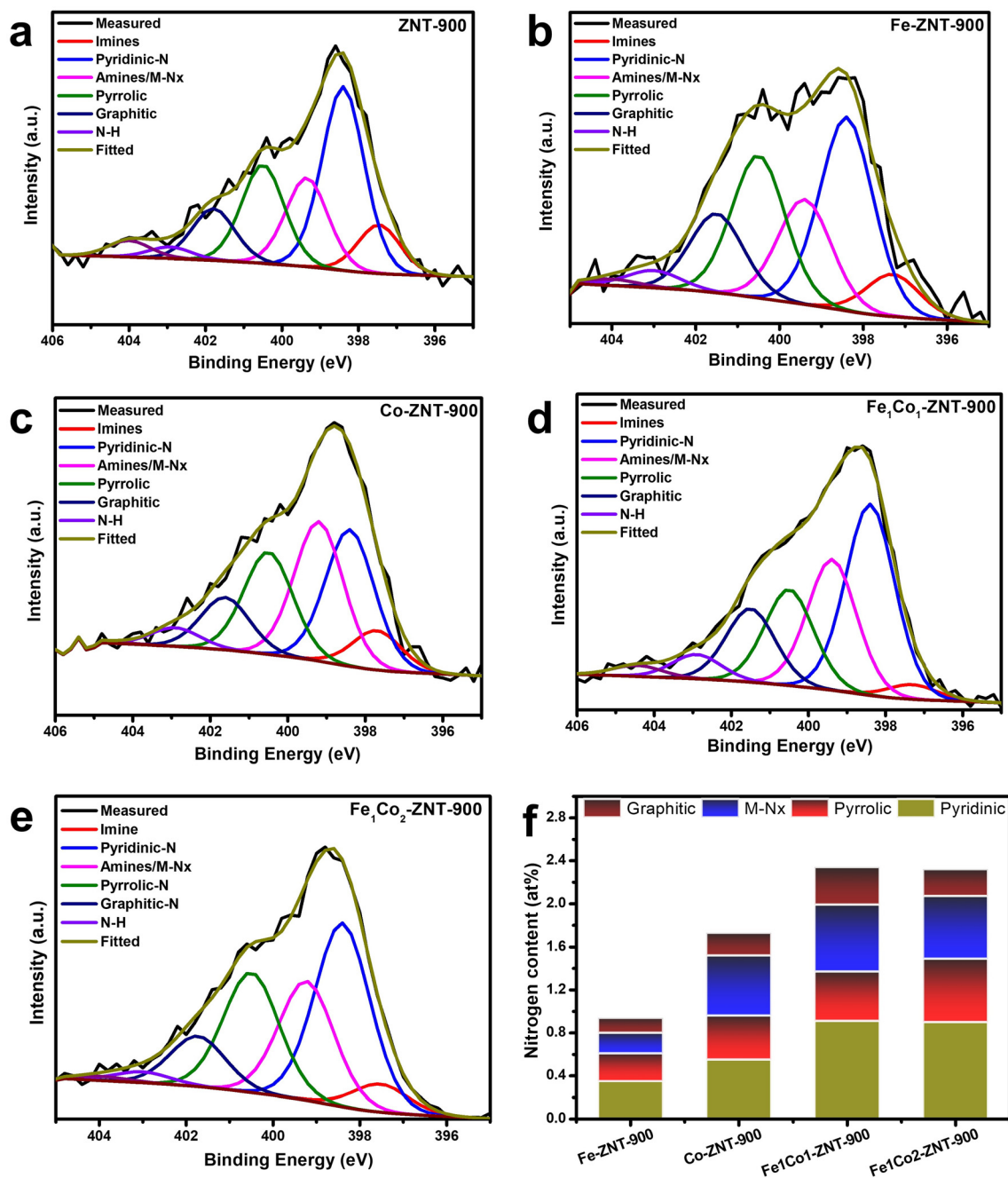
Fig. 5 (a–e) Comparison of N 1s XPS spectra for (a) ZNT-900, (b) Fe-ZNT-900, (c) Co-ZNT-900, (d) \text{Fe}_1\text{Co}_1 -ZNT-900 and (e) \text{Fe}_1\text{Co}_2 -ZNT-900 catalysts and (f) N content for different nitrogen groups.
