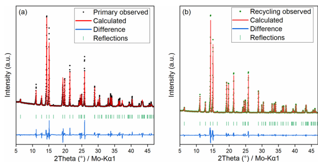
Fig. 4 Comparison of the Rietveld refinements of PXRD data ( \text{Mo}-K\alpha_1 ) for primary LCNC (a) and recycled LCNC (b). The theoretical reflections are also indicated for reference.
