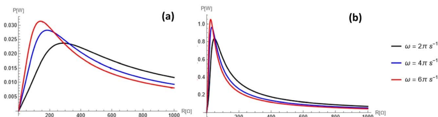
Fig. 11 Average power profile against the electric load for a porous electrode. Plotted for different external pressure frequencies at V_{\text{ref}} = 1.5 V where the pore radius r_p is (a) 10^{-5} m and (b) 10^{-7} m. Other parameters used are: \bar{C} = 5 \times 10^{-2} F m ^{-2} ; S_T = 0.002 m ^2 ; \varepsilon = 0.5 ; \theta_w = 131.18^\circ ; \eta = 6.3 \times 10^{-2} Pa s ^{-1} ; \gamma = 2.27 \times 10^{-2} N m ^{-1} .
