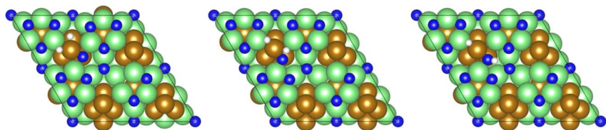
Fig. 11 Graphics illustrating the initial (left), transition (centre), and final (right) state geometries associated with the first N* hydrogenation process (Table 3, process 4).
