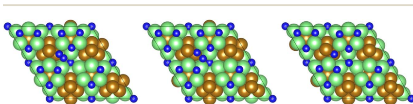
Fig. 10 Graphics illustrating the initial (left), transition (centre), and final (right) state geometries associated with N_2 dissociation (Table 3, process 2).
