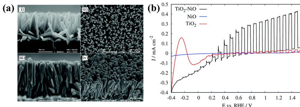
Fig. 30 (a) Scanning electron microscopy images of TiO 2 nanorods before (above) and after (below) NiO ALD coating, (b) photocurrent densities measured under chopped 1 sun rear-side illumination for TiO 2 , NiO, and NiO-coated TiO 2 systems. Reproduced with permission from ref. 327 copyright 2021, Royal Society of Chemistry.
