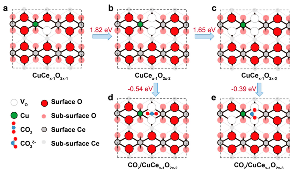
Fig. 10 (a–c) Structural diagrams of Cu doped \text{CeO}_2 , with 1–3 \text{V}_\text{o} . (d and e) \text{CO}_2 adsorption and activation structural diagrams of these structure. Reproduced with permission. 87 Copyright (2018) American Chemical Society.
