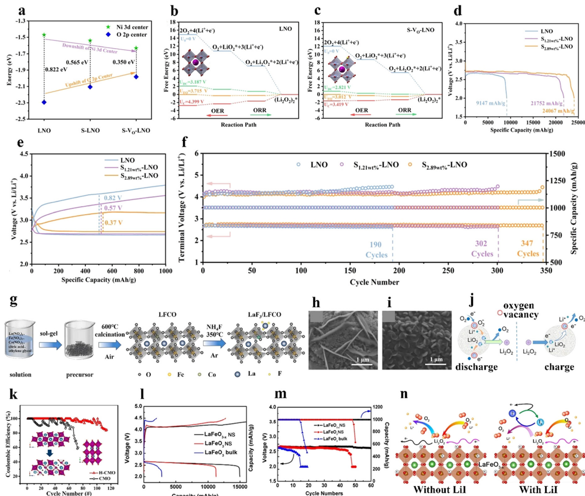
Fig. 6 The impact of B-site substitution and oxygen vacancies on perovskites. (a) Illustration of Ni 3d and O 2p band centers S-Vo-LNO and control samples. Free energy diagram of the ORR on (b) LNO and (c) S-Vo-LNO. (d) Discharge curves at 100 \text{ mA g}^{-1} , (e) discharge/charge curves with a confined capacity of 1000 \text{ mA h g}^{-1} at 100 \text{ mA g}^{-1} . (f) Cycling stability of the LOBs with LNO and S-Vo-LNO cathodes. (a)–(f) Reproduced with permission. 68 Copyright 2022, Elsevier. (g) Illustration of the synthesis process of LaF 3 /LFCO. SEM images of (h) LFCO and (i) LaF 3 /LFCO cathodes after the first discharge. (g)–(i) Reproduced with permission. 69 Copyright 2022, Elsevier. (j) Formation and decomposition processes of Li 2 O 2 on N-doped LNO during the discharge/charge process. Reproduced with permission. 70 Copyright 2018, American Chemical Society. (k) Coulombic efficiency of H-CMO and CMO. Insets: Their crystal structures. Reproduced with permission. 45 Copyright 2020, American Chemical Society. (l) The initial capacity at 100 \text{ mA g}^{-1} and (m) cycling stability of LaFeO 3 and LaFeO 3-x . (n) ORR and OER mechanisms on the LaFeO 3-x surface with/without Lil. (k)–(n) Reproduced with permission. 76 Copyright 2020, Elsevier.
