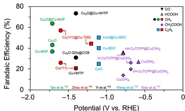
Fig. 23 Maximum faradaic efficiencies for CO, HCOOH, CH 4 , CH 3 COOH, and C 2 H 4 production for various Cu MOF composites compared to that of their constituent metallic and Cu MOF catalysts in the same experimental setup. QDs = quantum dots. CCB = conductive carbon black.
