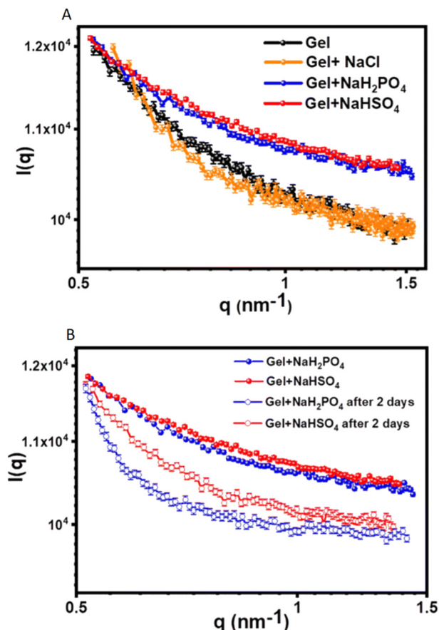
Fig. 6 SAXS scattering plots produced from the analysis of the NapF-TREN hydrogel: (A) before and after the addition of \text{Cl}^- , \text{H}_2\text{PO}_4^- and \text{HSO}_4^- ions, supplied as the sodium salt; (B) showing the effect of material ageing. Reproduced/adapted from ref. 61 with permission from RSC Nanoscale .
