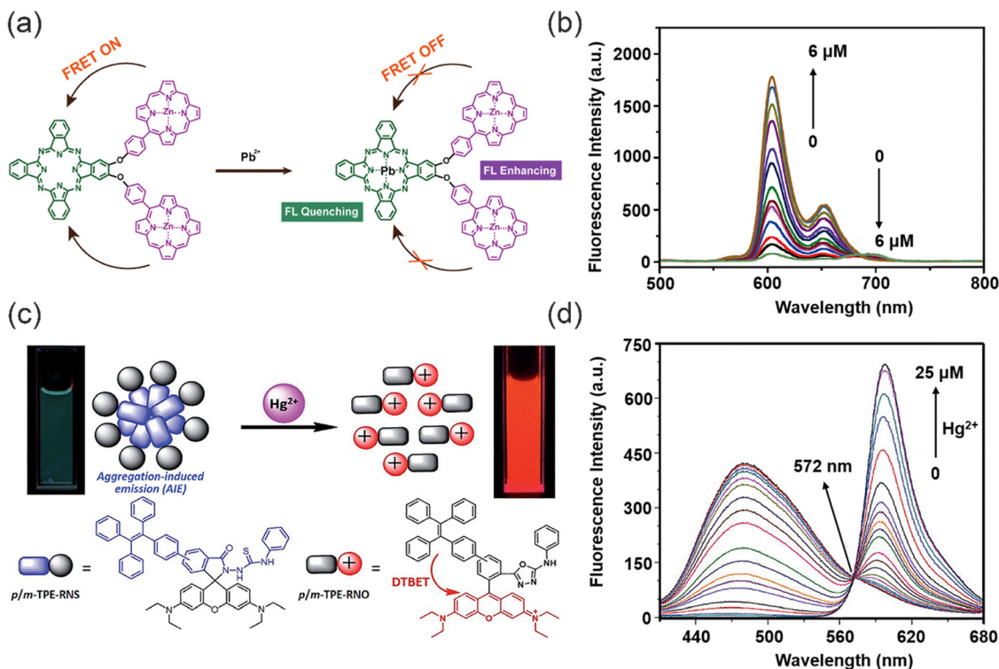
Fig. 5 The synthesis of “ratiometric” fluorescent probes and their fluorescence spectra for detecting heavy metal ions. (a) The sensing mechanism of ratiometric probe for Pb 2+ . (b) fluorescence spectra of triad 1 upon addition of Pb 2+ . Reproduced from ref. 49 with permission from Elsevier Ltd. Copyright 2019. (c) The sensing mechanism of p/m-TPE-RNS for Hg 2+ . (d) Fluorescence spectra of 10 mM m-TPE-RNS under different concentrations of Hg 2+ . Reproduced from ref. 50 with permission from Royal Society of Chemistry. Copyright 2017.
