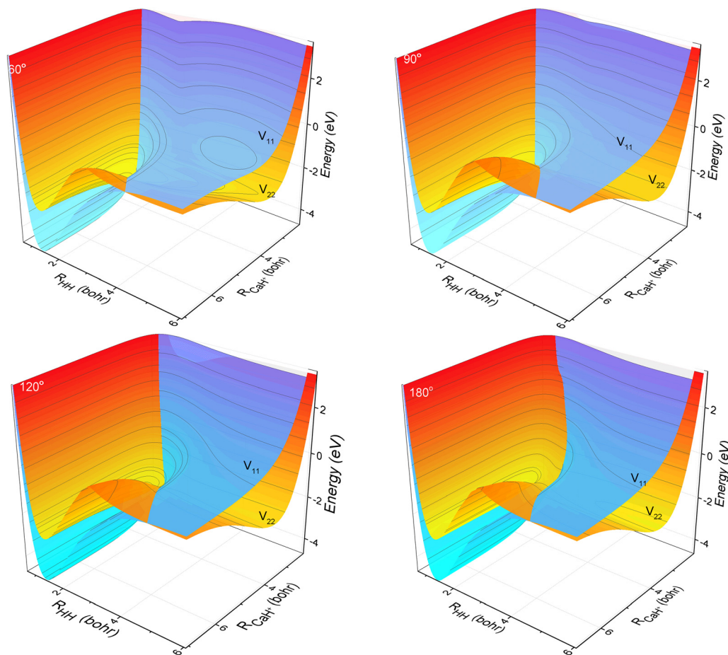
Fig. 1 3D PESs of the non-adiabatic states V_{11}^{11} and V_{22}^{22} for Ca-H-H with bond angles of 60.0°, 90.0°, 120.0° and 180.0°.
