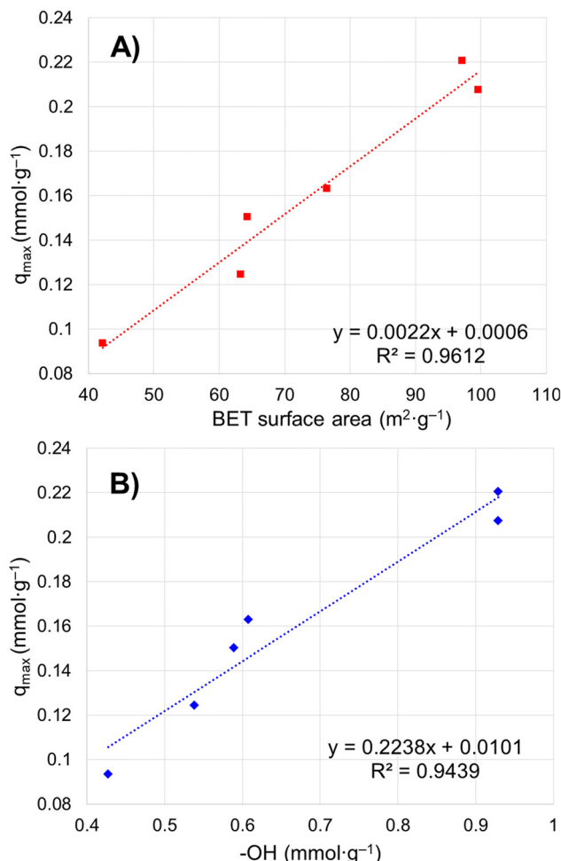
Fig. 8 Relation between maximum uranyl adsorption capacity and (A) particulate specific surface area by BET modelling; (B) -\text{OH} concentration on particle surface.
