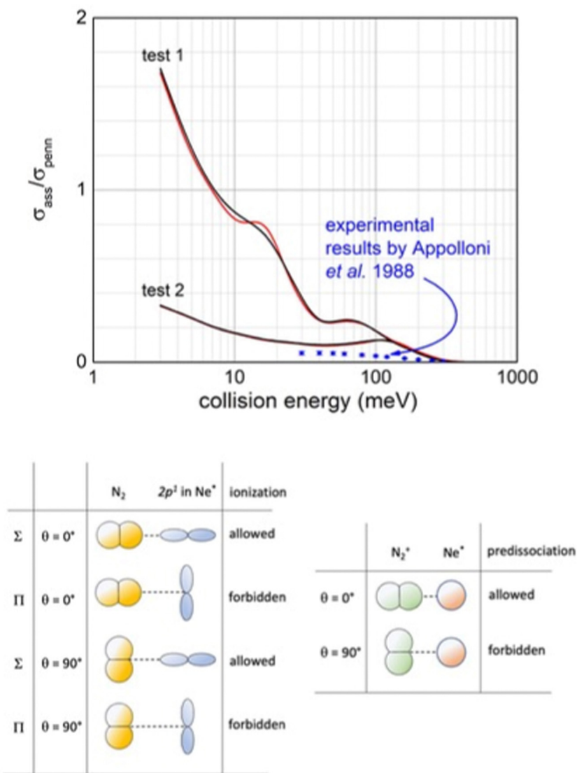
Fig. 16 Upper panel: Comparison, as a function of the collision energy, between predicted associative/Penning ratio for Ne*( 3 P 2 ) (red line) and Ne*( 3 P 0 ) (black line) reagents and data measured 127 using a statistical population of atomic fine levels. Lower panel: Schematic view of precursor state structures promoting reaction and associated ion formation. Note that while the HOMO orbital of N 2 , from which the electron is removed, does not exhibit any nodal plane perpendicular to the bond axis (passing for its centre of mass), the half-filled p orbital of Ne* atom exhibits a nodal plane. 119 Therefore, in all configurations characterized by overlap null between orbitals exchanging the electron, as in the second and fourth cases, the ionization by direct mechanism is forbidden and the reaction can occur only by an indirect mechanism (see text). Moreover, associate ions are efficiently formed, without pre-dissociation, only if N 2 maintains the perpendicular configuration both in the entrance and exit channels.
