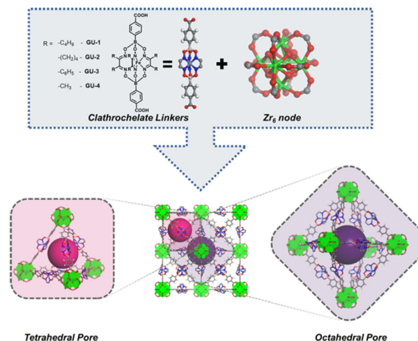
Scheme 1 Synthetic scheme of Zr-clathrocholate MOFs Zr-GU-1 to -4 and formation of octahedral and tetrahedral cavities within the framework.
