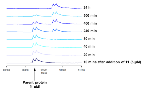
Fig. 12 Reaction of 11 with recombinant PI4KIII \beta .
