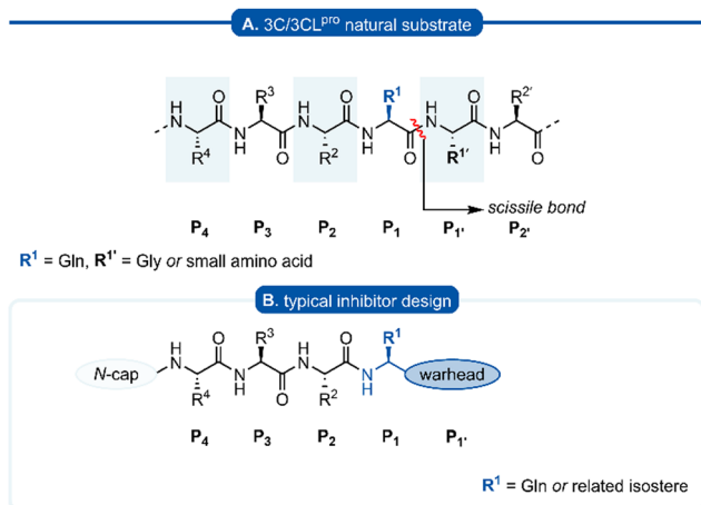
Fig. 1 (A) Hexapeptide recognition sequence of 3C/3CL P , where the scissile bond is located between P 1 (Gln) and P 1 * . (B) Typical inhibitor design targeting 3C/3CL P .
