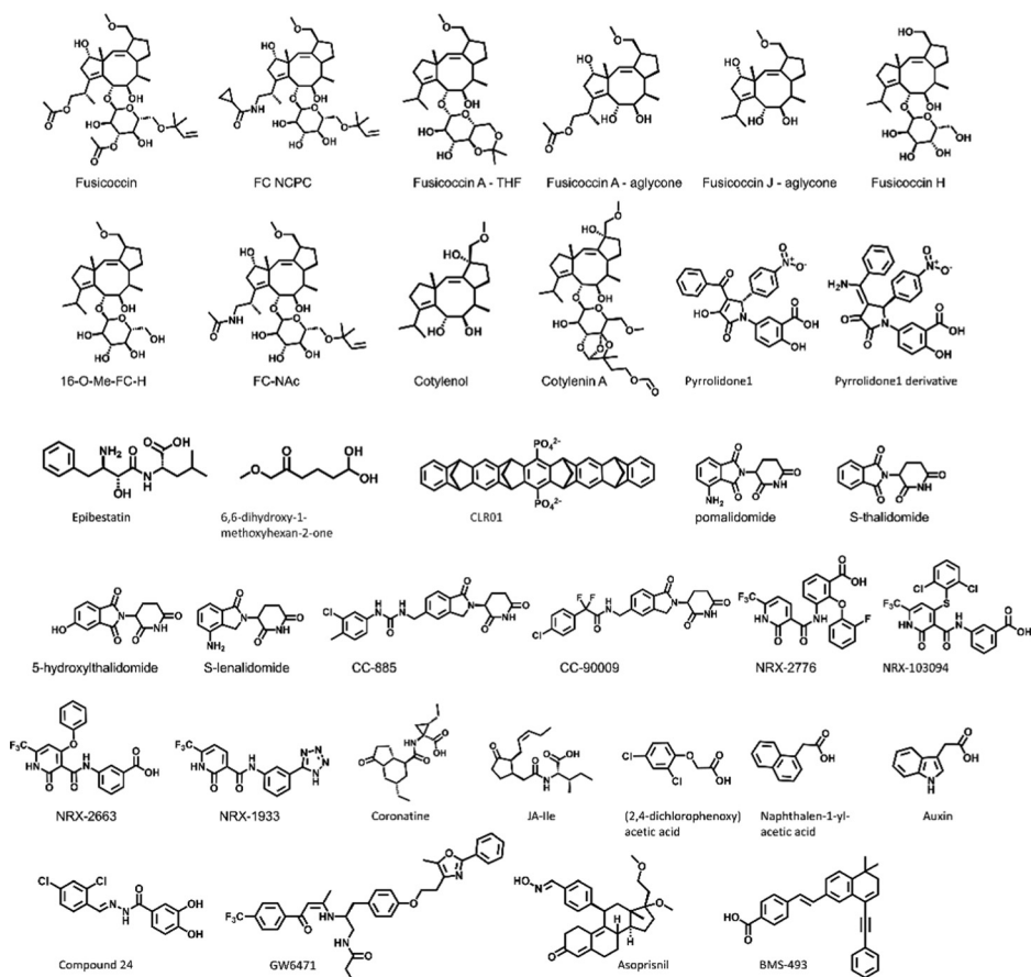
Scheme 1 All molecular glues in Table 1.
