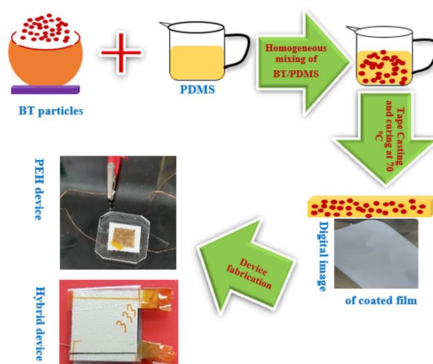
Fig. 5 Processing steps of the \text{BaTiO}_3 piezoceramic/PDMS composite and PEH/hybrid (PEH + TEH) device fabrication.
