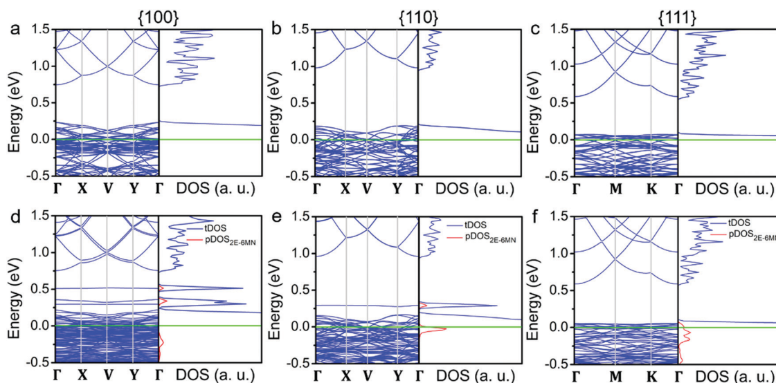
Fig. 8 (a–c) Band structures and density of states for the three different Cu 2 O crystallographic surfaces and (d–f) 2E-6MN-modified surfaces. Fermi level (green line) is set at zero in all band structures and density of states. The red peaks are the partial density of states (pDOS) from 2E-6MN molecules.
