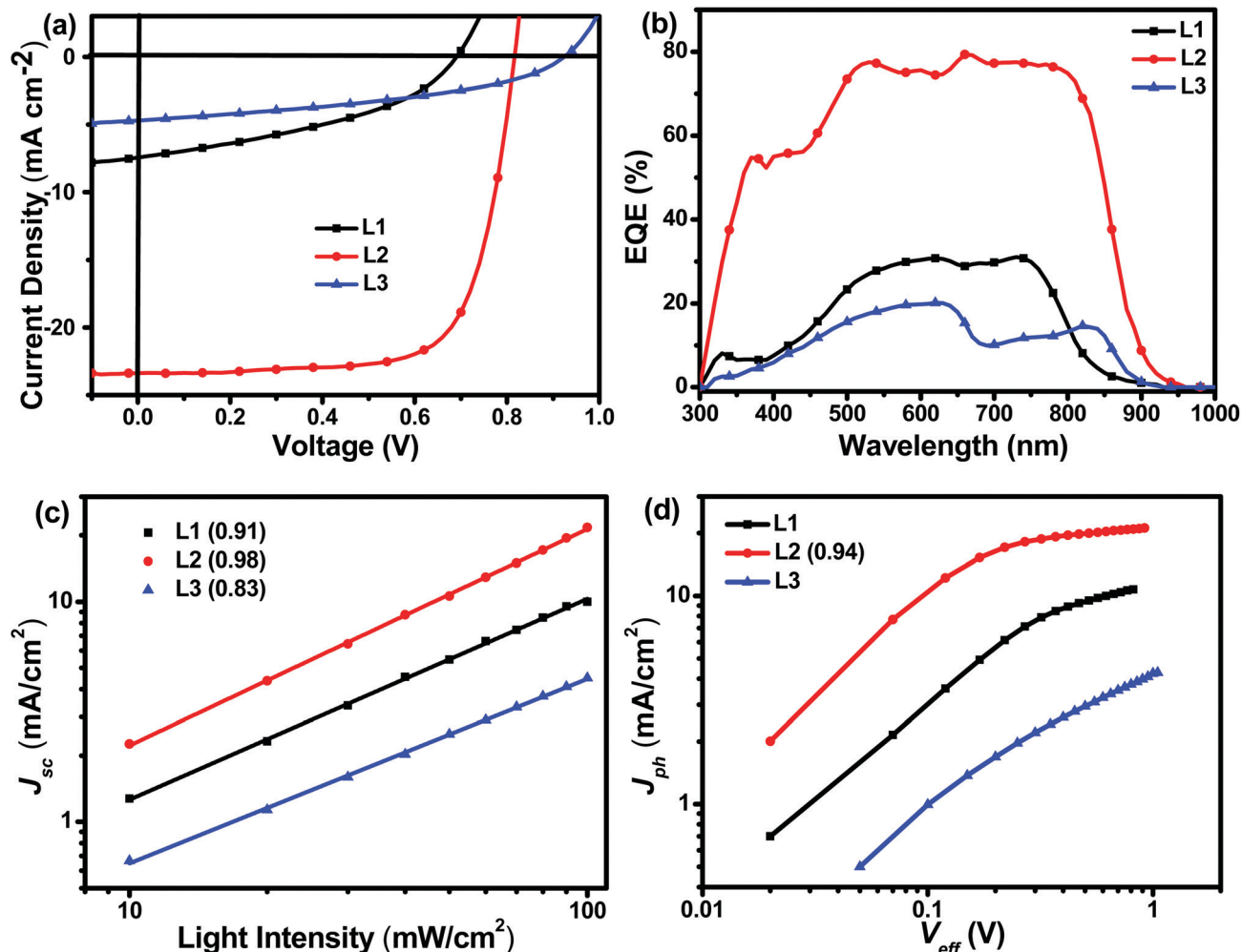
Fig. 3 (a) J - V and (b) EQE curves of L1-, L2-, and L3-based devices, (c) the dependence of J_{sc} on P_{\text{light}} and (d) the dependence of J_{ph} on V_{eff} .
