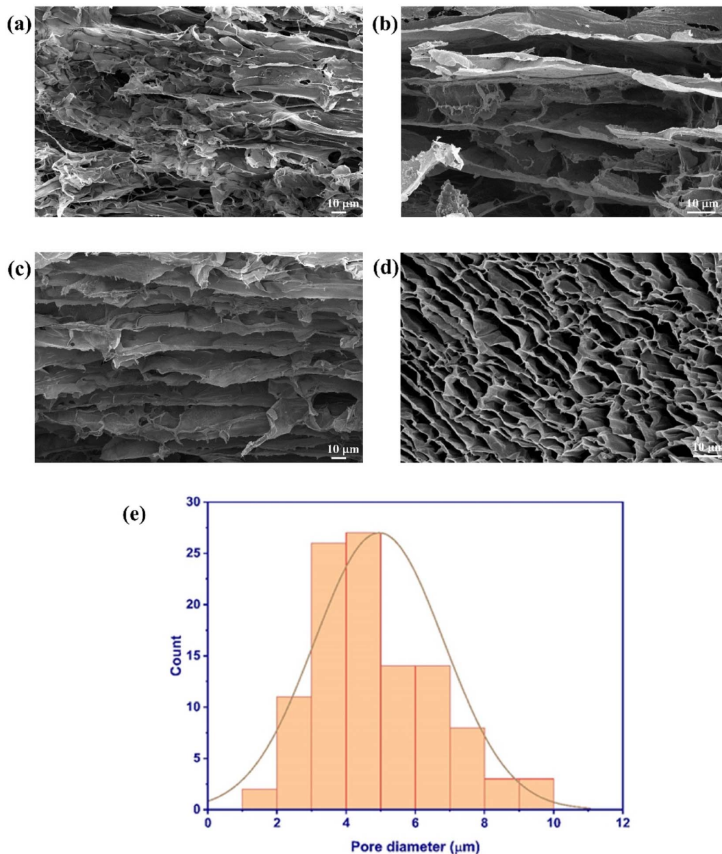
Fig. 7 FE-SEM of longitudinal structure of (a) Ref., (b) CMT, (c) CPMT cryogels; (d) cross-section of CPMT cryogel, and (e) average pore diameter of the CPMT cryogel.
