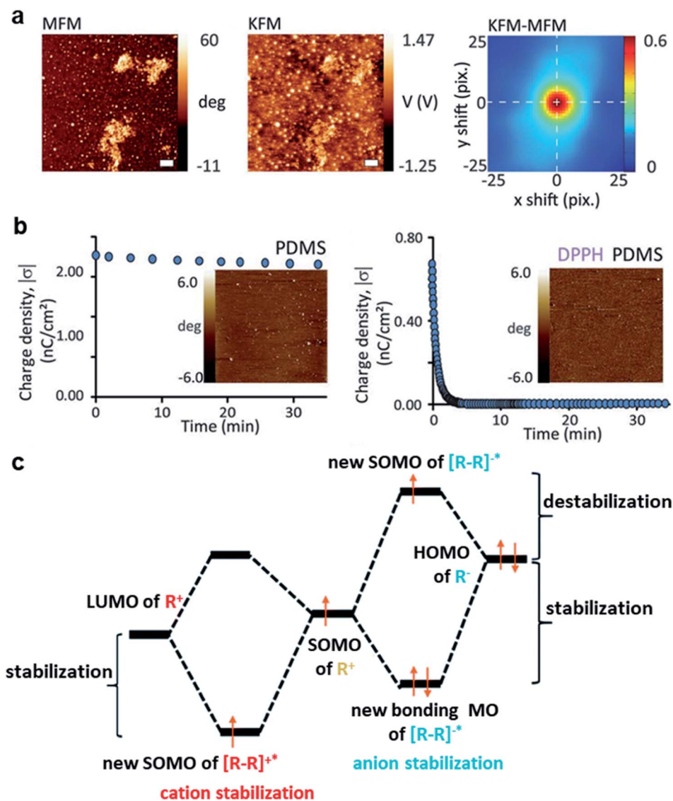
Fig. 7 Charge dissipation by removing the stabilizing radicals on the surface. (a) KFM and MFM images at the same location of a contact-charged surface of PDMS showing the co-localization of surface charge and radicals. (b) A surface doped with a radical scavenger ( i.e. , DPPH; plot on the right) in PDMS dissipated charge much faster than the undoped surface of PDMS (plot on the left). (a and b) Reproduced with permission (copyright 2013, American Association for the Advancement of Science). 20 (c) Proposed mechanism of radicals stabilizing cations and anions, reproduced with permission (copyright 2017, Royal Society of Chemistry). 113
