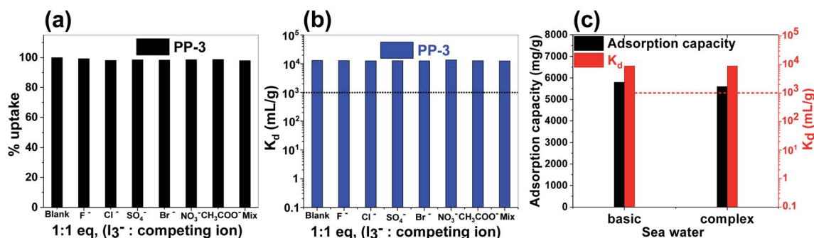
Fig. 7 (a) Uptake percent for \text{I}_3^- anions in the presence of other competing anions, (b) distribution coefficient ( K_d ) graph and (c) \text{I}_3^- adsorption capacity from the basic and complex seawater and the corresponding distribution coefficient value ( K_d ).
