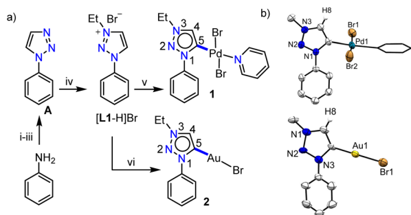
Scheme 1 (a) Synthesis of [L1-H]Br and its palladium ( 1 ) and gold ( 2 ) complexes: (i) NaNO_2 , HCl/H_2O (10% solution), 0 °C, 1 h; (ii) NaN_3 , 0 °C-RT, 12 h; (iii) vinyl acetate, reflux, 24 h; (iv) EtBr , CH_3CN , reflux, 24 h; (v) [Pd(CH_3CN)_2Cl_2] , CS_2CO_3 , KBr , CH_3CN /pyridine, 70 °C, 24 h; (vi) [Au(SMe_2)Cl] , CS_2CO_3 , CH_3CN , 70 °C, 24 h; (b) molecular structures of 1 and 2 with ellipsoids at a 50% probability level. Hydrogen atoms except H8 and Me moieties of the N-Et groups are omitted for clarity. Pyridine is shown in capped stick.
