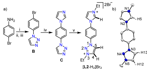
Scheme 2 (a) Synthesis of bisazolium salt, [L2-H_2]Br_2 : (i) NaNO_2 , HCl/H_2O (10% solution), 0 °C, 1 h; (ii) NaN_3 , 0 °C-RT, 12 h; (iii) vinyl acetate, reflux, 24 h; (iv) imidazole, K_2CO_3 , CuO , DMSO , 150 °C, 48 h; (v) EtBr , DMF , reflux, 24 h. (b) Molecular structure of [L2-H_2]Br_2 with ellipsoids at a 50% probability level. Hydrogen atoms except H5, H12, and H13, counterions, solvent of crystallization and Me moieties of the N-Et groups are omitted for clarity.
