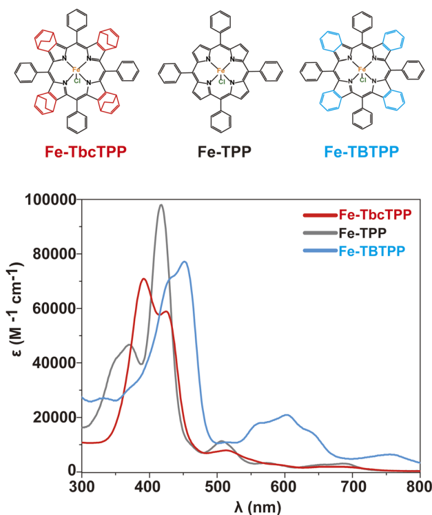
Fig. 1 The Fe-Por molecules synthesized and investigated as molecular catalysts in this study (top) along with the UV-vis spectra of the same in THF (bottom).
