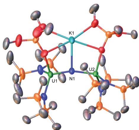
Fig. 3 Molecular structure of complex, [\text{K}\{\text{U}^{\text{IV/III}}(\text{OSi}(\text{O}^t\text{Bu})_3)(\text{N}(\text{SiMe}_3)_2)_2(\mu\text{-N})\}][\text{K}(\text{THF})_6] , 4, with thermal ellipsoids at drawn at the 50% probability level. Hydrogen atoms, methyl groups on the \text{OSi}(\text{O}^t\text{Bu})_3 ligands, and the [\text{K}(\text{THF})_6] cation have been omitted for clarity.
