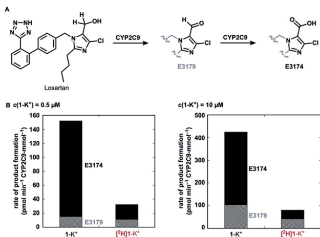
Fig. 6 (A) Metabolic pathway of losartan and (B) kinetic data on the formation of metabolites E3179( -d_1 ) and E3174 from 1\text{-K}^+ or [^2\text{H}]1\text{-K}^+ (96% D) by CYP2C9 under non-competitive intermolecular conditions.
