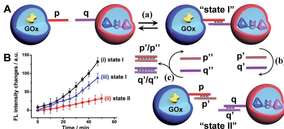
Fig. 6 (A) Switchable inhibition of the intercommunicated microcapsule GOx//hemin/G-quadruplex biocatalyst cascade using a “fuel” inhibiting strands p' , q' and “counter-fuel strands” p'' , q'' . (B) Time-dependent fluorescence changes corresponding to Resorufin generated by the intercommunicated GOx//hemin/G-quadruplex bridged T_1/T_2 cascade as a result of (a) equilibrated p/q interlinked microcapsule dimers, state I, curve (i). (b) Upon separation of the dimers using p' and q' fuel strands, state II, curve (ii), and (c) upon treatment of the separated capsules, state II with the counter fuel strands p'' and q'' to regenerate state I, curve (iii). Error bars derived from N = 3 experiments.
