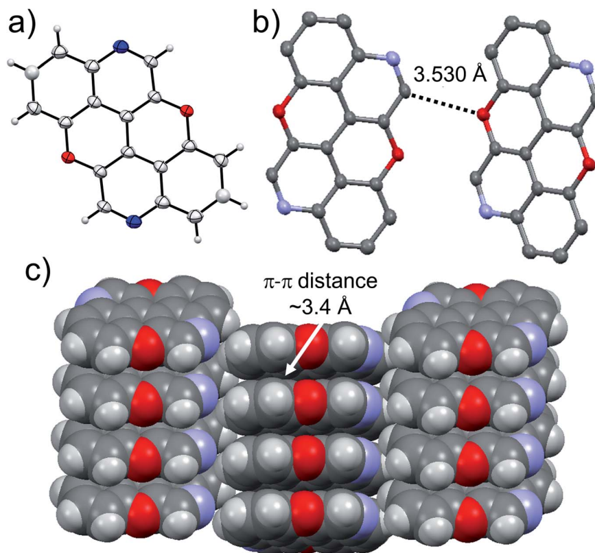
Fig. 10 Single-crystal X-ray structure of 4,10- N,N -PXX. ORTEP representation (a) and structure of two molecules engaging into H-bonds (b) forming a columnar organization (c). Space groups: P2_1/n . Atom colours: red O, blue N, grey C, white H.
