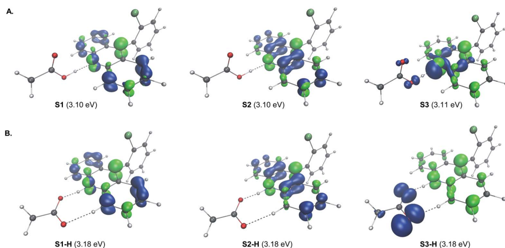
Fig. 4 Electron–hole analysis of the three lowest singlet excited states of the hydrogen bond complex of acridine A1 and acetic acid before (A) and after (B) the O → N proton transfer.
