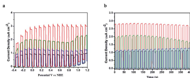
Fig. 5 (a) Photocurrent density–voltage ( j – v ) traces with 5 s light transients for \text{TiO}_2|\text{TPA}|\text{PNO} (red), \text{TiO}_2|\text{TPA} (green), \text{TiO}_2|\text{TPA}|\text{Nafion} (blue) and \text{TiO}_2|\text{TPA}|\text{PMMA} (black) scanned from -0.4 to 1.2 V vs. NHE with a scan rate of 1 \text{ mV s}^{-1} under 1 sun illumination in pH 7, 0.1 \text{ M} phosphate buffer containing 0.1 \text{ M Na}_2\text{SO}_3 . (b) The time dependent photopotential density ( j – t ) traces with 10 s light transients at 0.4 \text{ V} vs. NHE.
