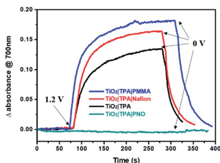
Fig. 4 Absorption changes at 700 nm associated with time-dependent oxidation of \text{TiO}_2/\text{TPA}/\text{PMMA} (blue), \text{TiO}_2/\text{TPA}/\text{Nafion} (red), \text{TiO}_2/\text{TPA} (black) and \text{TiO}_2/\text{TPA}/\text{PNO} (green) in pH 7, 0.1 M phosphate buffer containing 0.4 M \text{NaClO}_4 following a potential step from 1.2 to 0 V vs. NHE.
